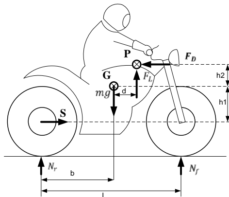
Fig. 1 Fundamental forces applied to the test bike
